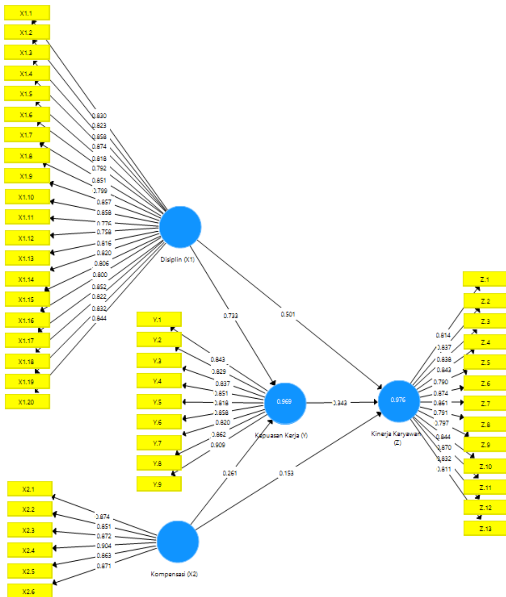
Gambar 1. Outer Loading
