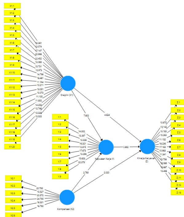
Gambar 2. Bootstraping
